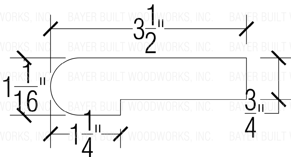
8090 LANDING TREAD
